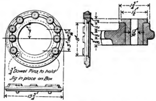
Figs. 4771-4774. Standard Jig for Boring Trailing Truck Boxes.
